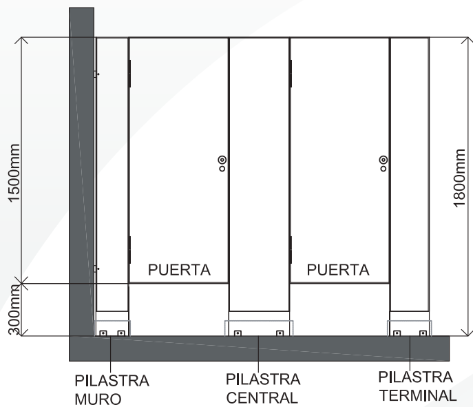
VISTA FRONTAL
